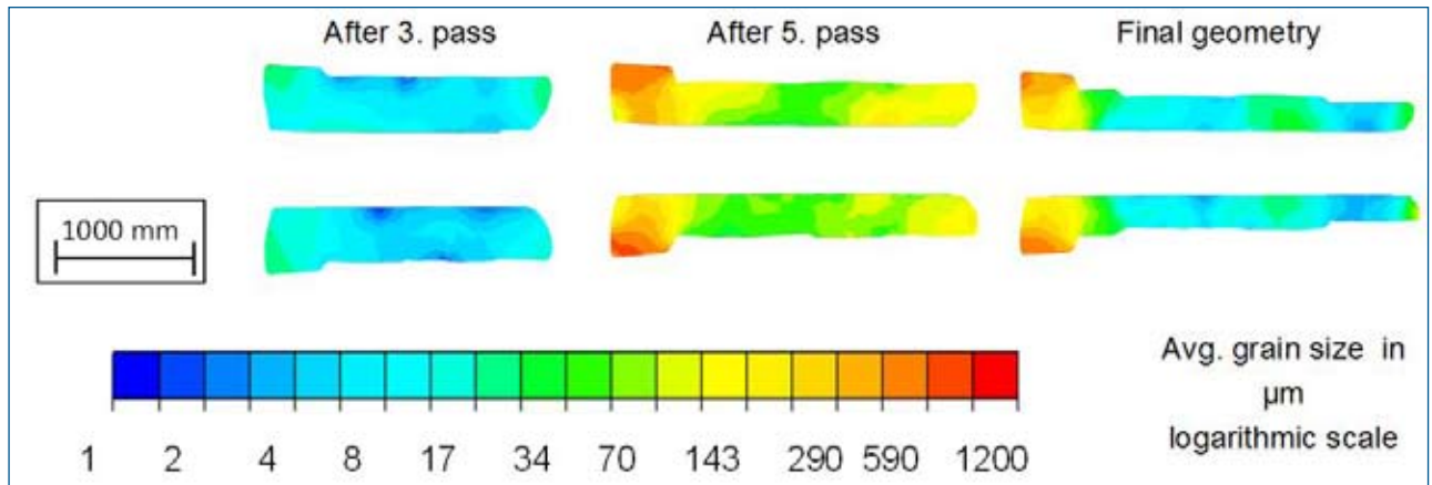
Fig. 9 - Grain size evolution for a hollow shaft with an industrial geometry (Reheating after 3rd pass)
