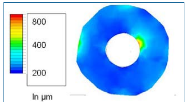
Fig. 4 - Exemplary grain size distribution at the cross section
